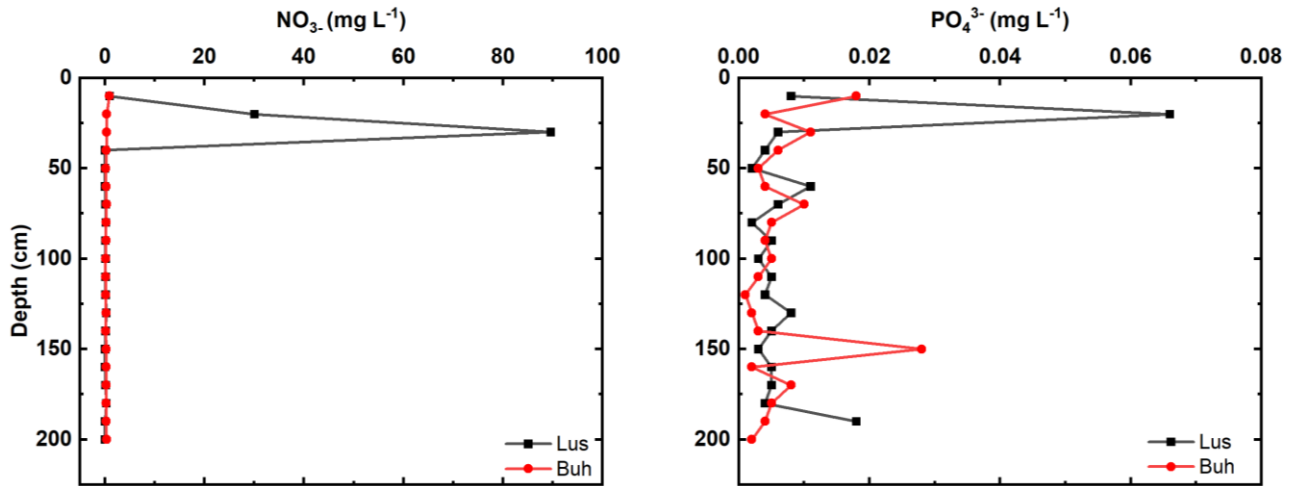
Figure 7. Profiles of nitrate ( \text{NO}_3^- ) and phosphate ( \text{PO}_4^{3-} ) for peat cores from the second (2018) campaign at Buhandanda (Buh) and Lushala (Lus).
