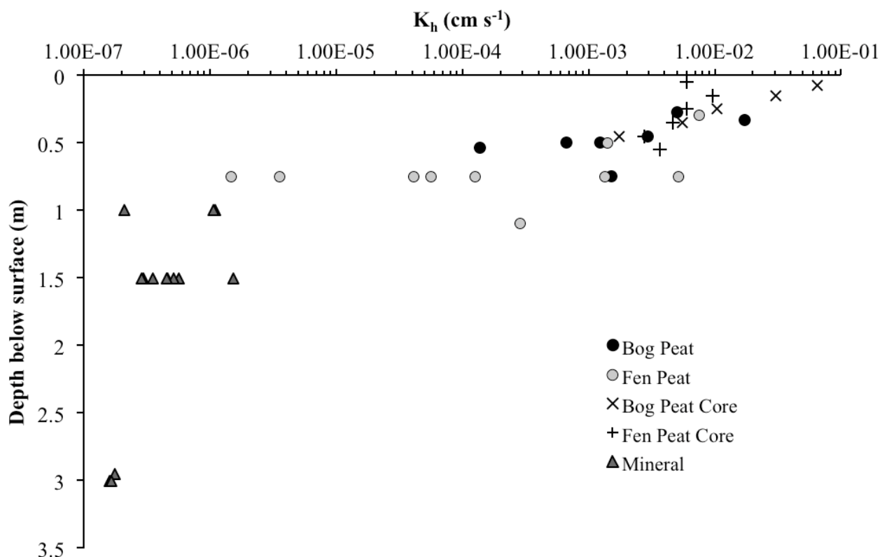
Figure 3. Saturated horizontal hydraulic conductivities ( K_h ) along T1, T2 and T3, calculated using the bail test method. K_h values, measured in the laboratory on the bog (T1-BM) and fen (T1-FM) peat cores, are also shown.
