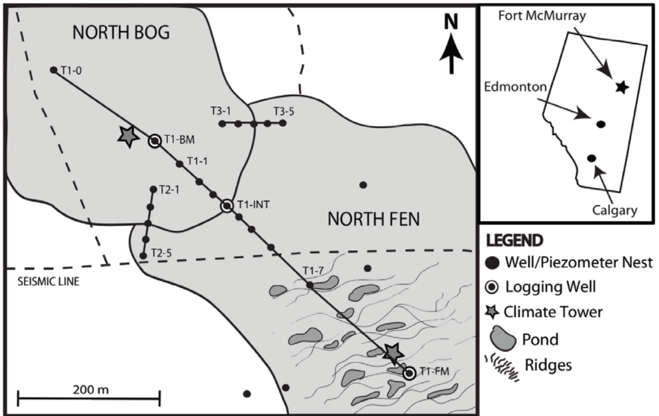
Figure 1. Map of the saline fen / bog study area located within the WBP of north-eastern Alberta (inset) ~18 km south of Fort McMurray (modified from C. Wells 2013, unpublished data).
