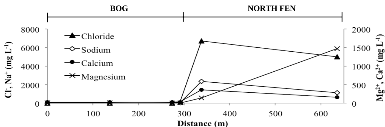
Figure 5. Groundwater chemistry along T1, measured from T1-0 to T1-FM. The values are averages of measurements from the June and August sampling periods where available.
