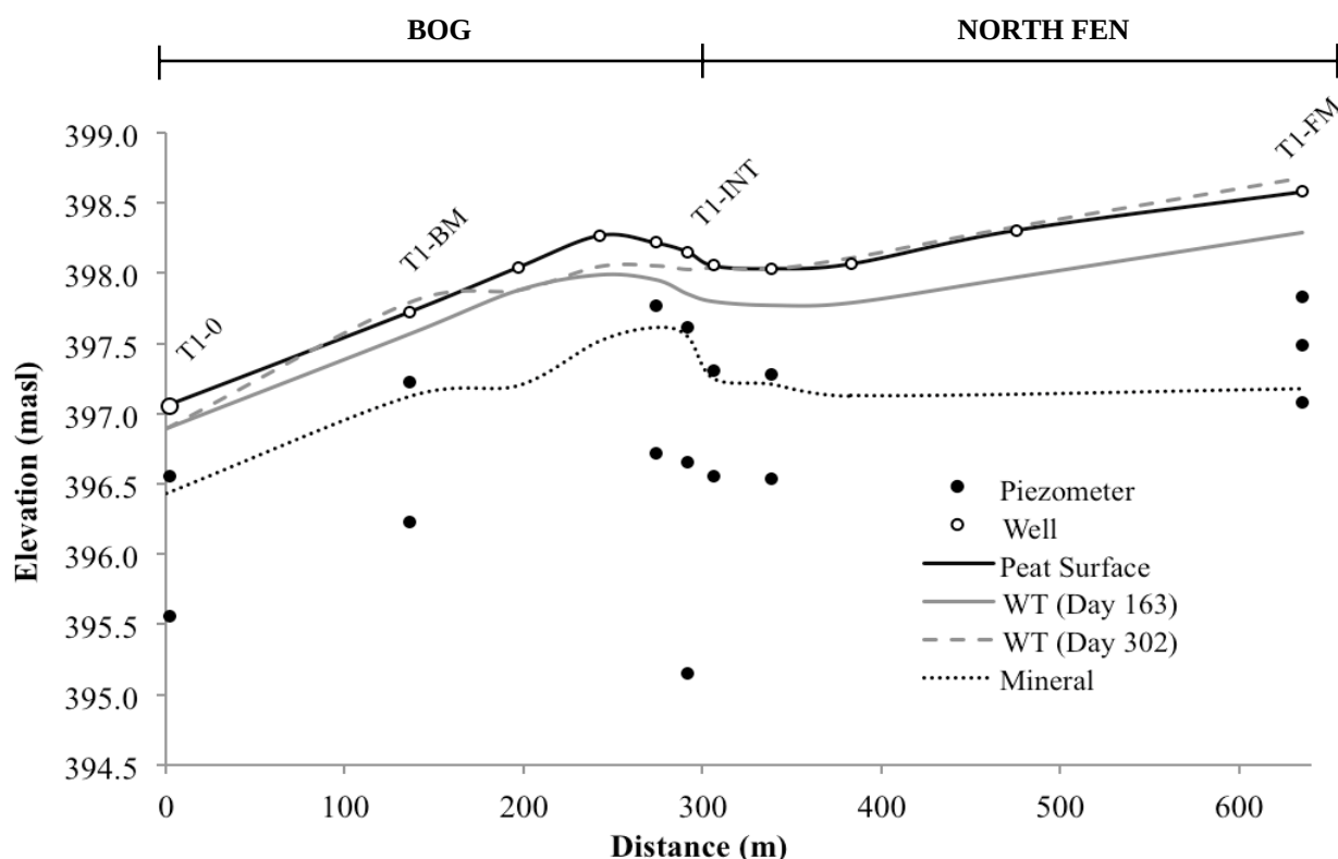
Figure 2. Stratigraphy and water table position along T1, measured from T1-0 (0 m) to T1-FM (635 m), showing water table position during a dry period (Day 163) and a wet period (Day 302).
