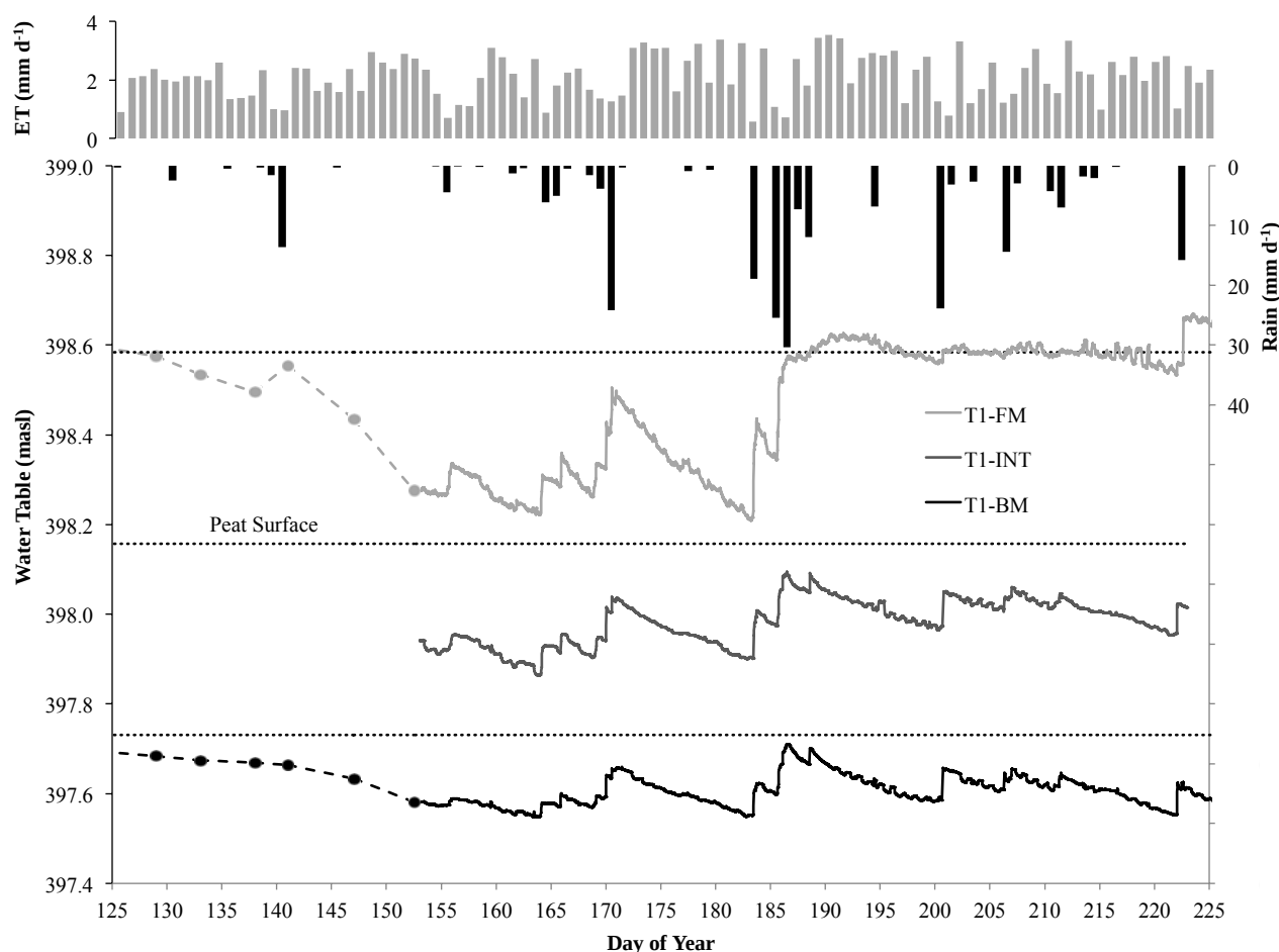
Figure 4. Water table position along T1, with the respective ground surface altitudes associated with each (dotted lines), from May 4 (Day 125) to August 12 (Day 225). Solid lines indicate continuous water level measurements and dashed lines indicate manual measurements. There were no manual measurements prior to June 01 (Day 153) for T1-INT. Daily P and ET , calculated from the bog meteorological station data, are plotted for the same time period.
