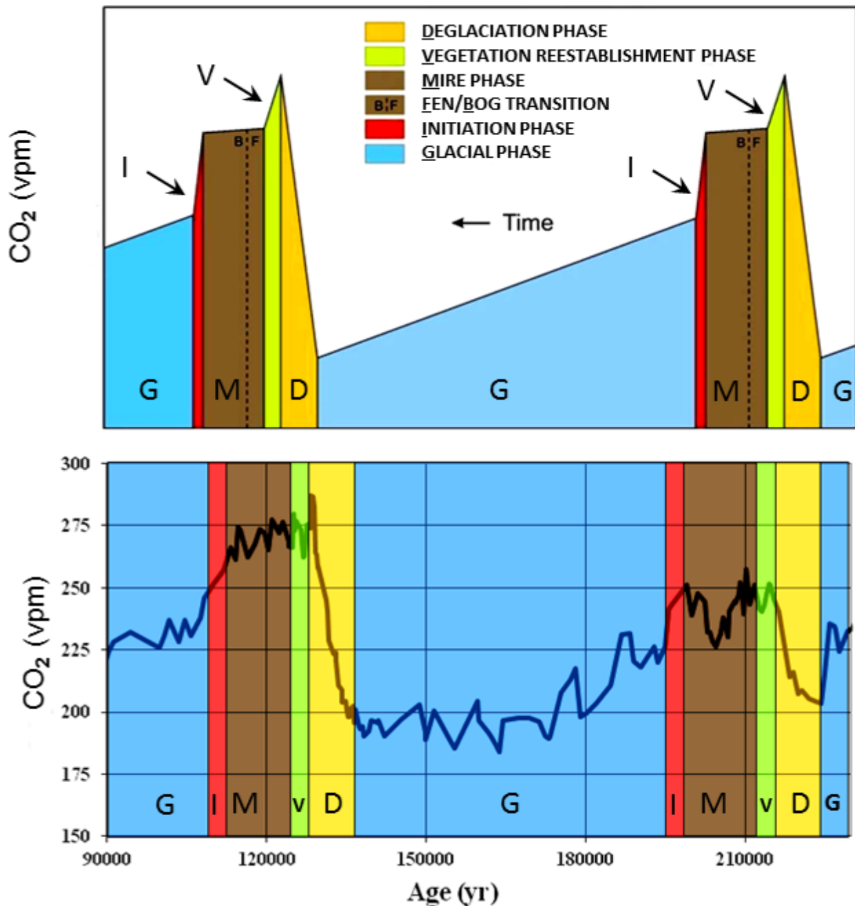
Figure 1. The idealised \text{CO}_2 development of age cycles according to the P/IAH (above) and applied to the \text{CO}_2 concentrations of 90–230 kyr from Antarctic ice cores (Petit et al. 1999, Monnin et al. 2001, Pépin et al. 2001, Raynaud et al. 2005) (below).
