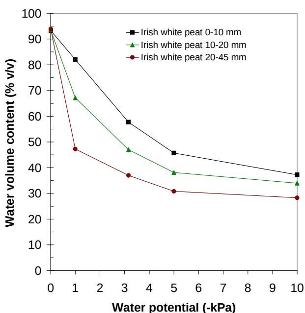
Figure 3. Examples of water retention curves of white Sphagnum peat with different particle size distributions.
