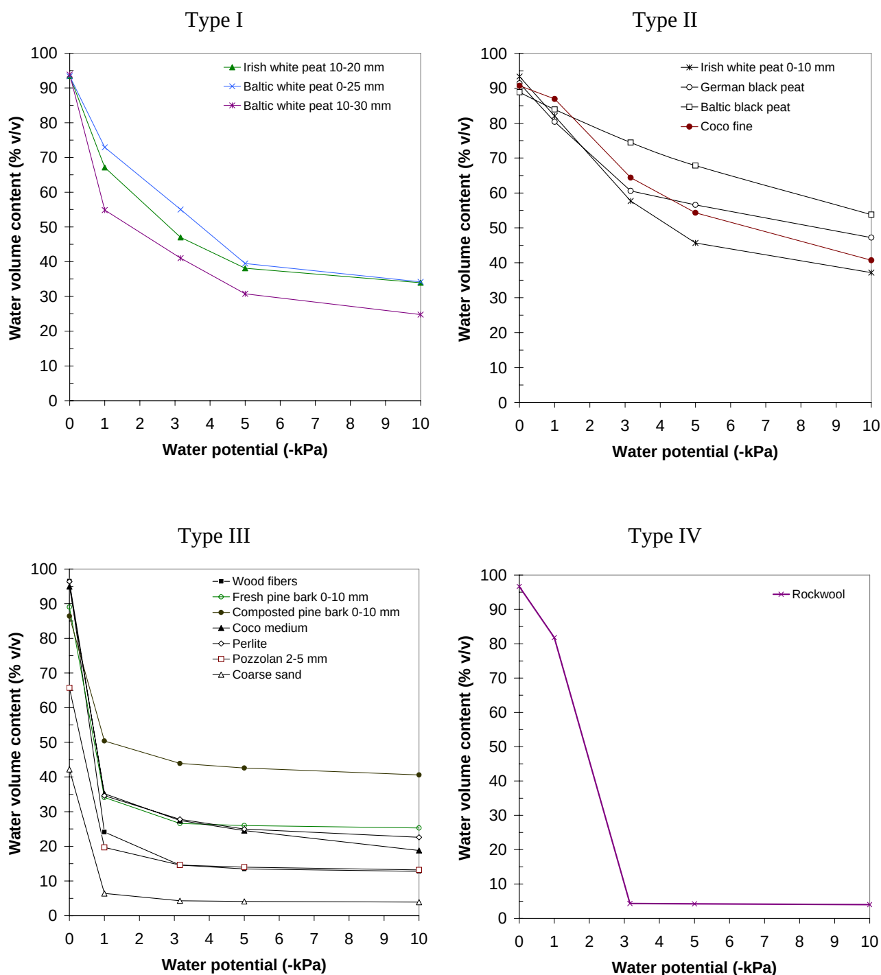
Figure 4. Examples of water retention curves for different materials used as growing media.
