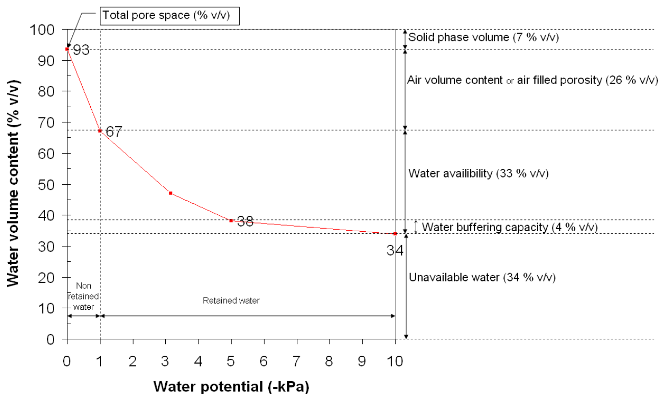
Figure 1. Key features of an example water retention curve.
