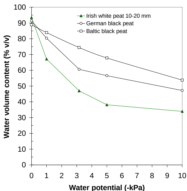
Figure 2. Examples of retention curves of different types of peat at various degrees of decomposition, and consequences in terms of physical characteristics.
