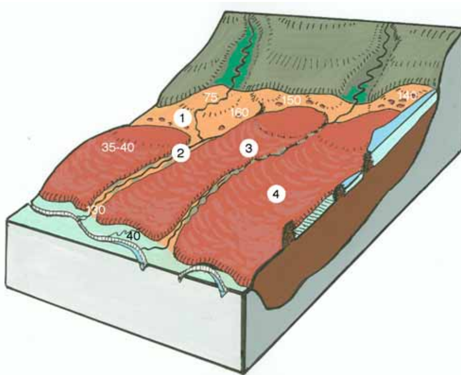
Figure 8. Sketch of the Andorra mire showing the EC values (in \mu\text{S cm}^{-1} ) measured in surface water (white digits) on 23 November 2005. The white circles indicate the locations where peat profiles were described. Sphagnum magellanicum bog is shown in red, fen in orange and open water in blue.
