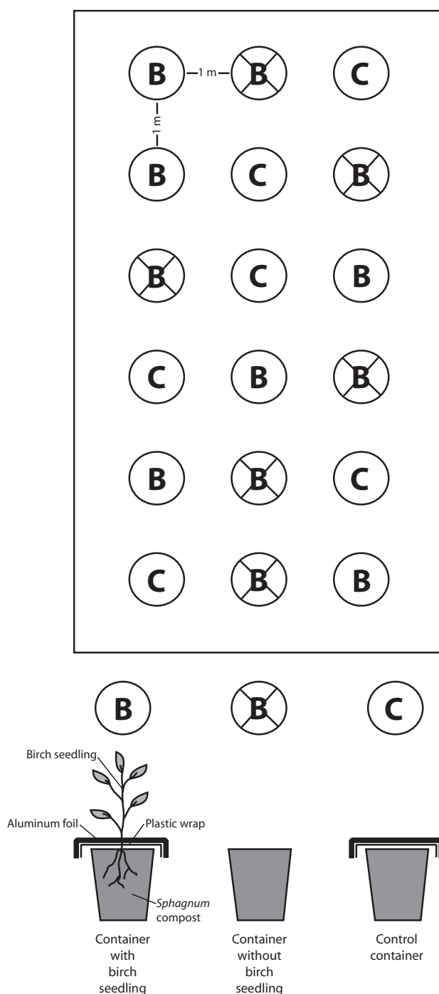
Figure 1. Example of the experimental set-up that was used to measure evaporation and transpiration rates at the Saint-Henri-de-Lévis peatland, southern Quebec, Canada, during the summer of 2005.
