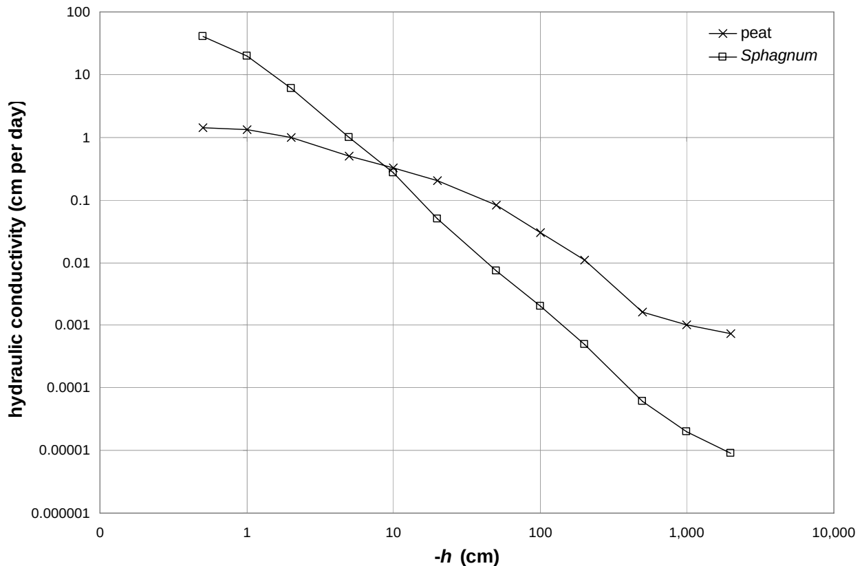
Figure 7. Relationship between unsaturated hydraulic conductivity k(h) and pore water pressure h for a Sphagnum moss layer (derived from literature and measurements) and of the underlying peat (measured) as used in the sensitivity analysis.
