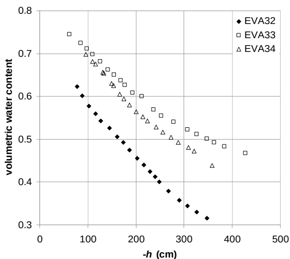
Figure 4. Water retention characteristics at low pore water pressure for three samples from a wet site with Sphagnum . Sample EVA32 was taken from depth 10–20 cm in slightly humified (H4–5) Sphagnum peat. Samples EVA33 and EVA34 were from a more humified (H6–7) layer (depth 35–45 cm) at the same location.
