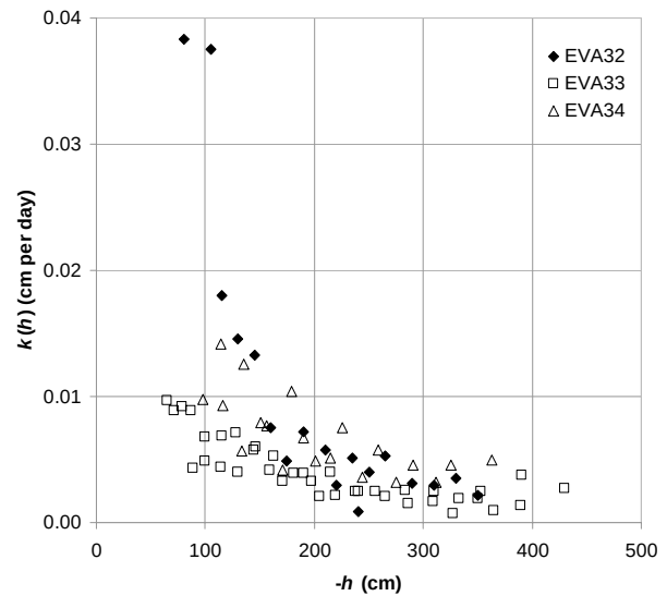
Figure 5. Relationships between unsaturated hydraulic conductivity k(h) and pore water pressure ( -h ) at low pore water pressure for three samples (EVA32–34 as for Figure 4) from a wet site with Sphagnum . Each point represents the average k(h) value for a 5 cm class of h .
