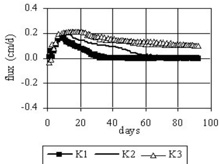
Figure 9. Variations in water flux 1 cm below the upper surface of a 2 cm thick Sphagnum moss layer during the simulation period 01 June – 31 August 1998 for the three site condition scenarios described in Figure 1. All simulations began with the moss layer saturated. Three different hydraulic conductivity ( k ) values are used for the peat underlying the Sphagnum layer: K1: k = 0.316 \times geometric mean value for Samples EVA32–34; K2: k = geometric mean value; and K3: k = 3.16 \times geometric mean value. Abscissae indicate the number of days from the start of each simulation.
