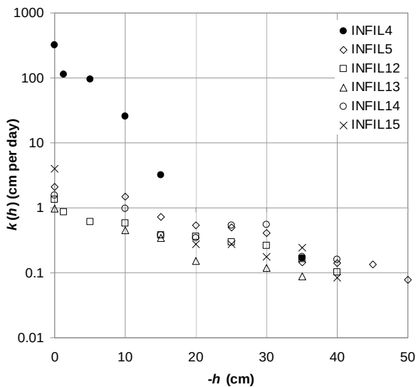
Figure 3. Relationships between hydraulic conductivity k(h) (logarithmic scale) and -h (absolute value of negative pore water pressure) determined using the 'infiltr' method for samples from a site dominated by Eriophorum angustifolium . Samples INFIL5 and 12–15 consisted of peat (H4–5 on the von Post scale) taken from depth 10–30 cm. Sample INFIL4 was taken from depth 0–20 cm in a living Sphagnum compactum cushion. The first (left-hand) value of k(h) in each series ( h = 0 ) indicates the saturated hydraulic conductivity. Values for h = -1.5 cm indicate the mean k(h) value for 0 > h > -2.5 cm. For values of h < -2.5 cm, each point represents the mean of all measured k(h) values corresponding to values of h within a 5 cm class.
