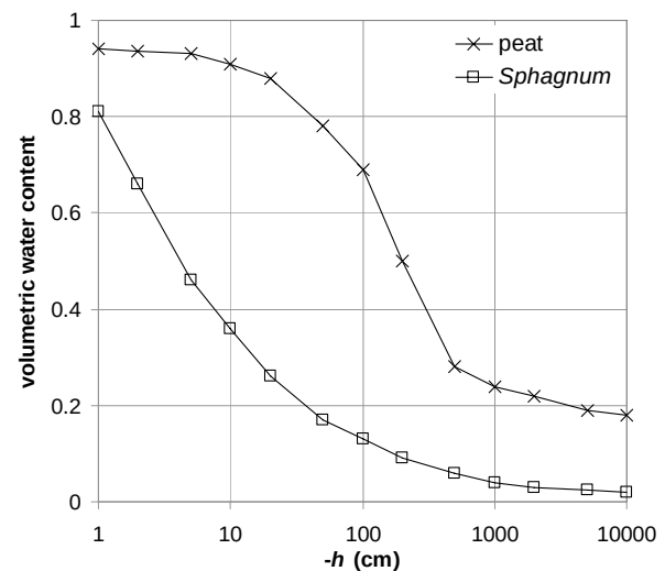
Figure 6. Water retention curves ( \Theta – h relationship) for a Sphagnum moss layer (derived from literature and measurements) and for the underlying peat (measured) as used in the sensitivity analysis.
