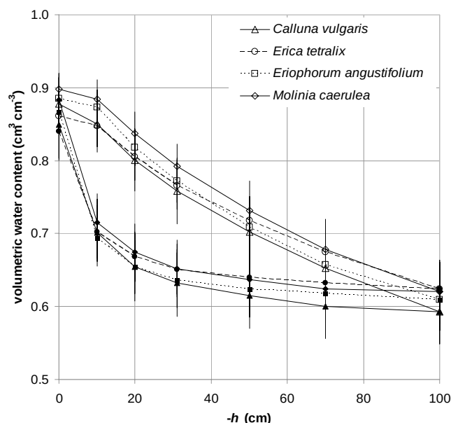
Figure 2. Water retention curves (mean values and standard deviation, n = 13 ) for peat samples taken from depth 5–10 cm beneath four different vegetation types, distinguished on the basis of dominant species. For each vegetation type, both the desorption (upper, hollow symbols) curve and the adsorption (lower, filled symbols) curve is shown.
